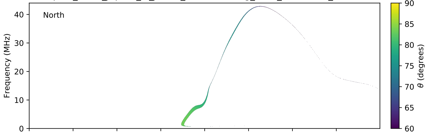
expres_earth_jupiter_io_jrm09_lossc-wid1deg_3kev_20100525_v01.cdf
