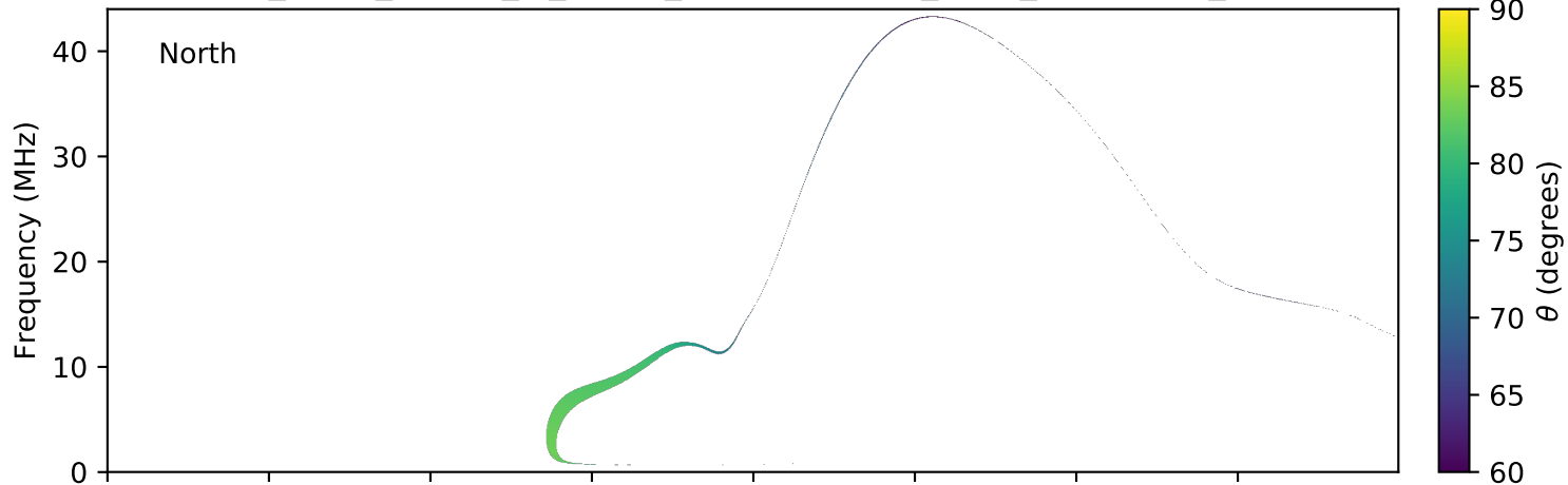
expres_earth_jupiter_io_jrm09_lossc-wid1deg_3kev_20100518_v01.cdf
