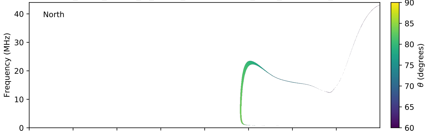
expres_earth_jupiter_io_jrm09_lossc-wid1deg_3kev_20100516_v01.cdf
