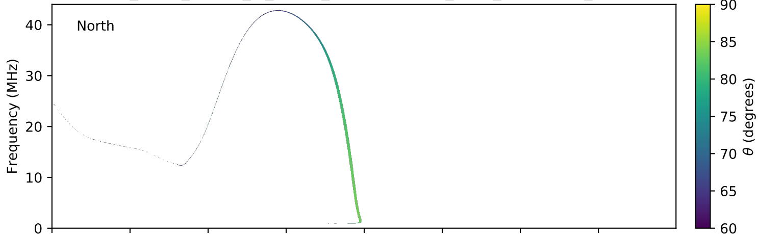
expres_earth_jupiter_io_jrm09_lossc-wid1deg_3kev_20100501_v01.cdf
