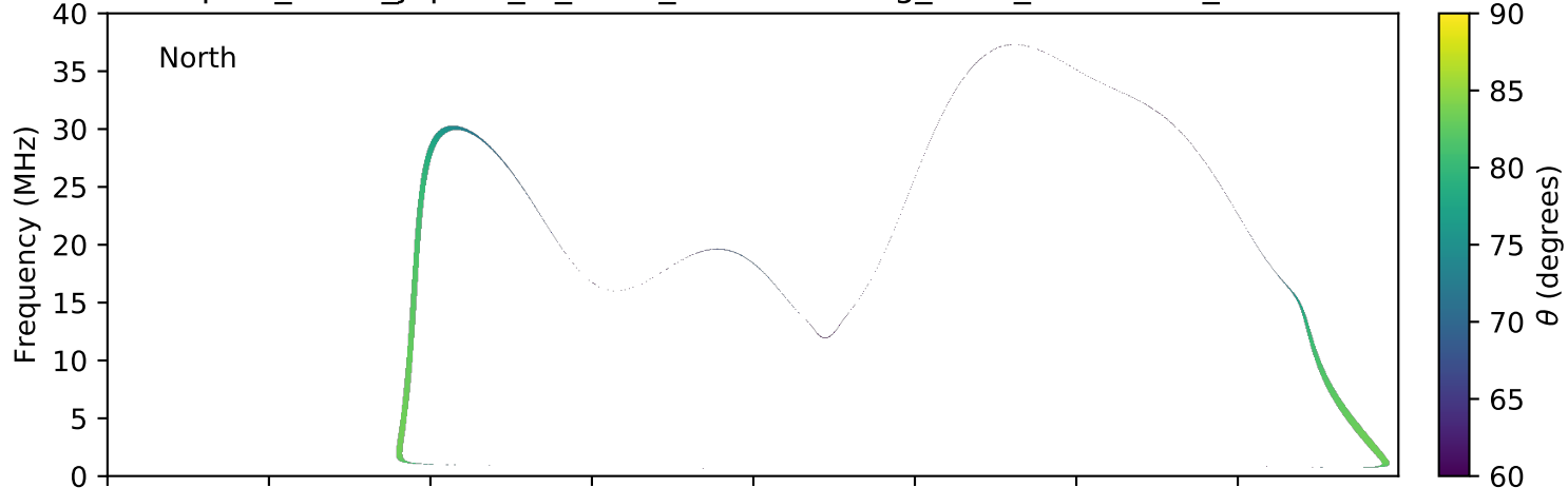
expres_earth_jupiter_io_isaac_lossc-wid1deg_3kev_20100527_v01.cdf
