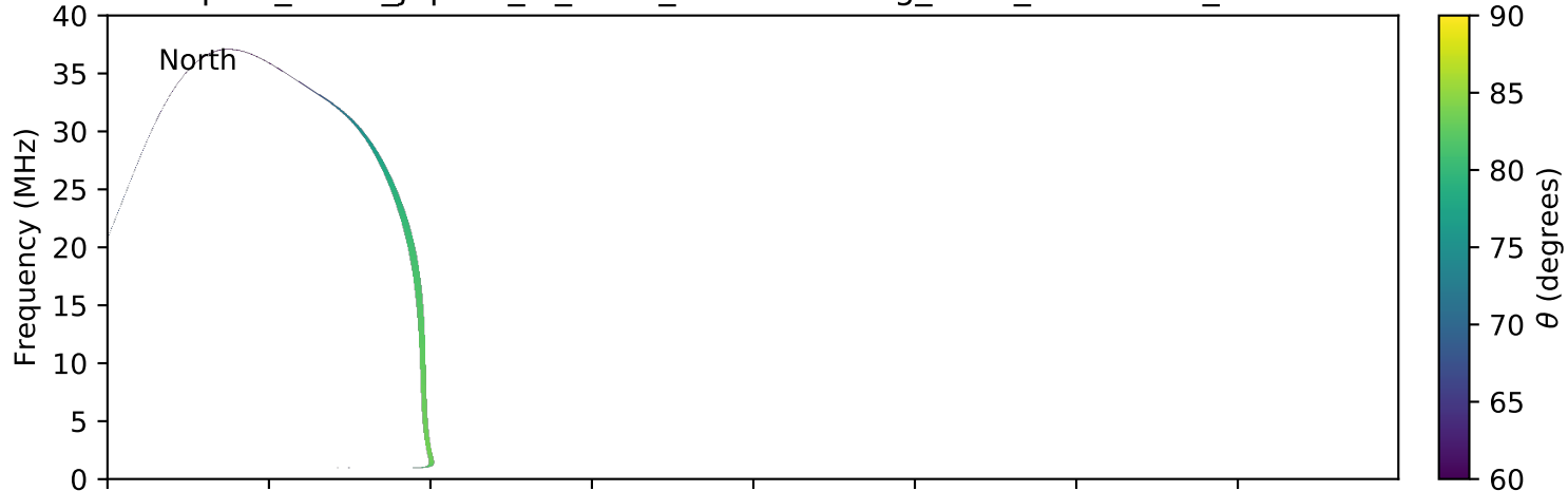
expres_earth_jupiter_io_isaac_lossc-wid1deg_3kev_20100526_v01.cdf
