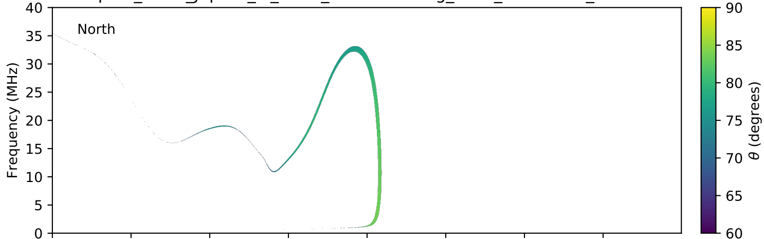
expres_earth_jupiter_io_isaac_lossc-wid1deg_3kev_20100524_v01.cdf
