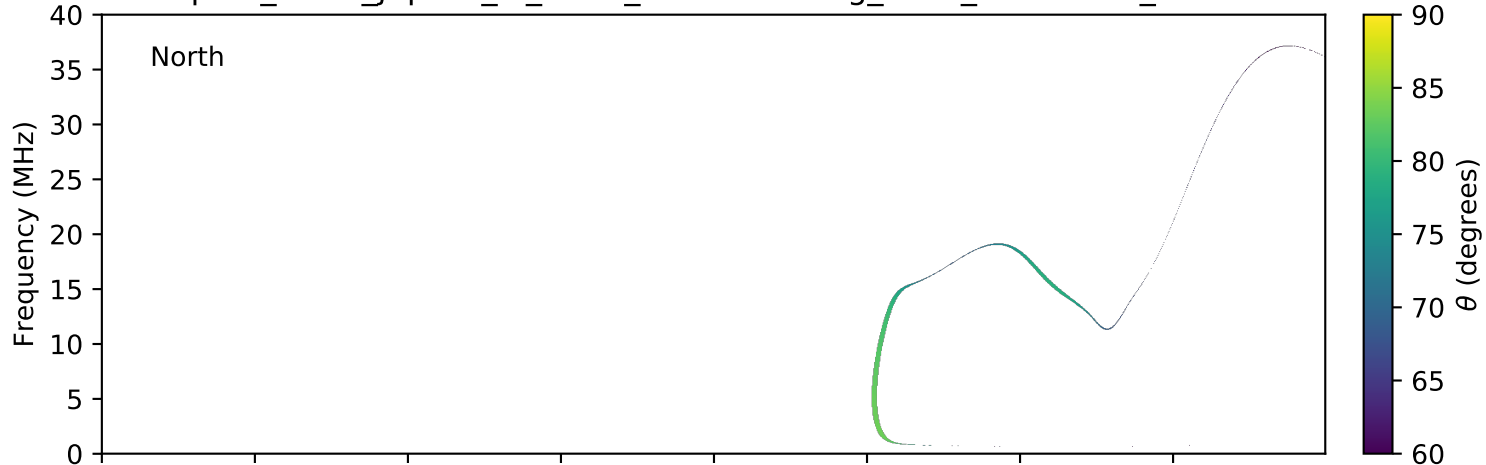
expres_earth_jupiter_io_isaac_lossc-wid1deg_3kev_20100523_v01.cdf
