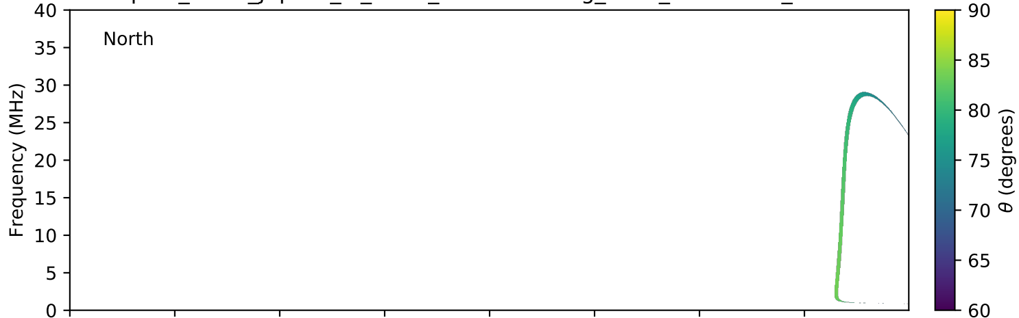
expres_earth_jupiter_io_isaac_lossc-wid1deg_3kev_20100521_v01.cdf
