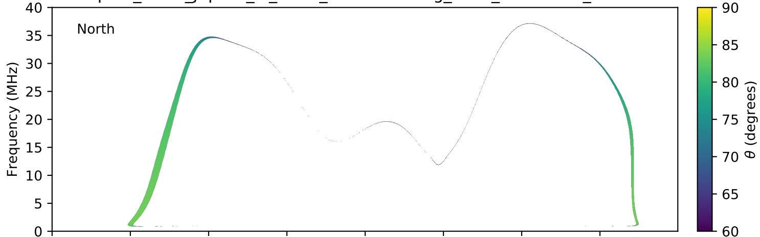
expres_earth_jupiter_io_isaac_lossc-wid1deg_3kev_20100520_v01.cdf
