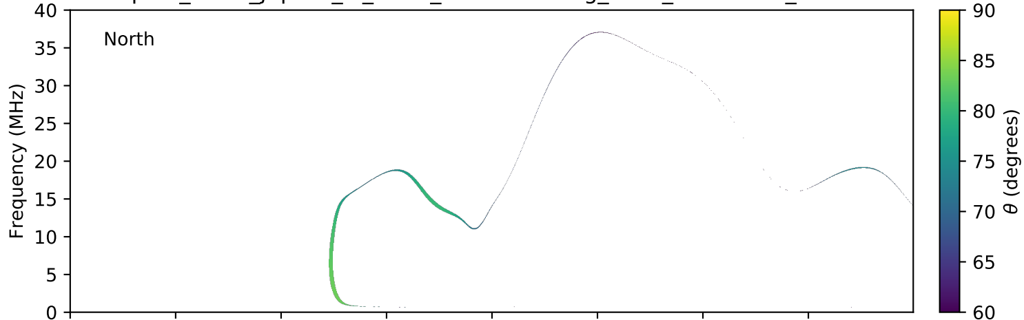
expres_earth_jupiter_io_isaac_lossc-wid1deg_3kev_20100518_v01.cdf
