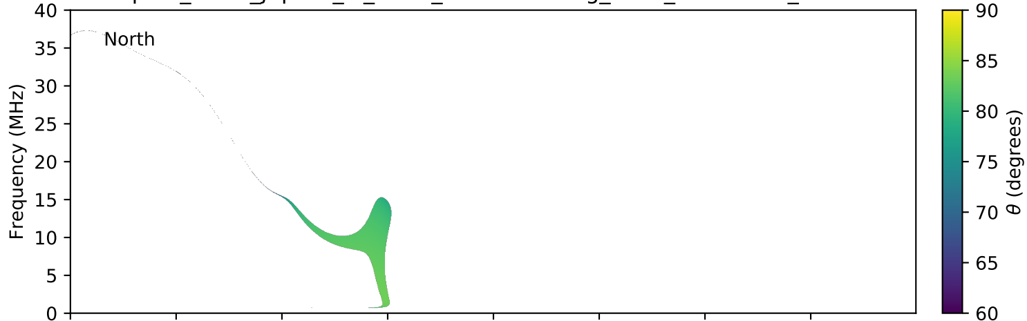
expres_earth_jupiter_io_isaac_lossc-wid1deg_3kev_20100517_v01.cdf
