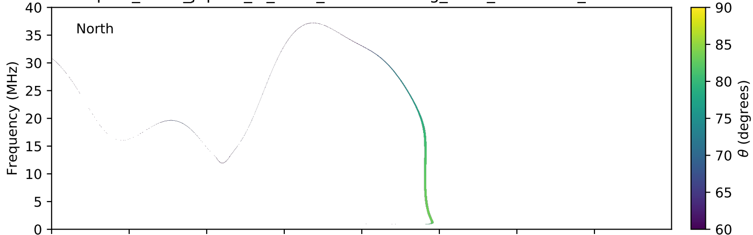
expres_earth_jupiter_io_isaac_lossc-wid1deg_3kev_20100515_v01.cdf
