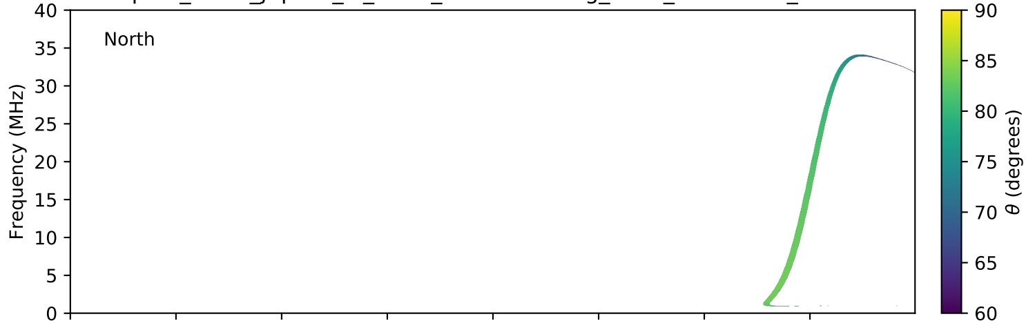
expres_earth_jupiter_io_isaac_lossc-wid1deg_3kev_20100514_v01.cdf
