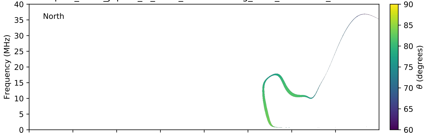
expres_earth_jupiter_io_isaac_lossc-wid1deg_3kev_20100507_v01.cdf
