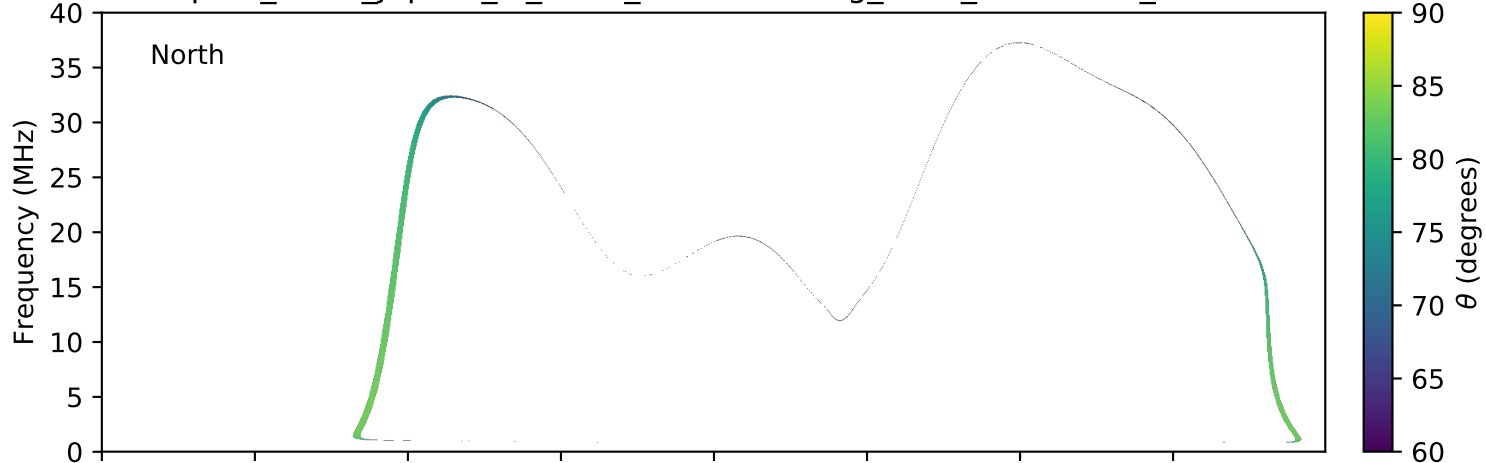
expres_earth_jupiter_io_isaac_lossc-wid1deg_3kev_20100504_v01.cdf
