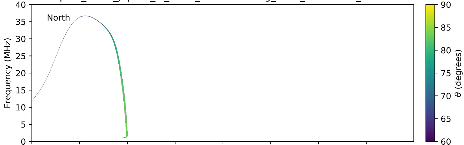
expres_earth_jupiter_io_isaac_lossc-wid1deg_3kev_20100503_v01.cdf
