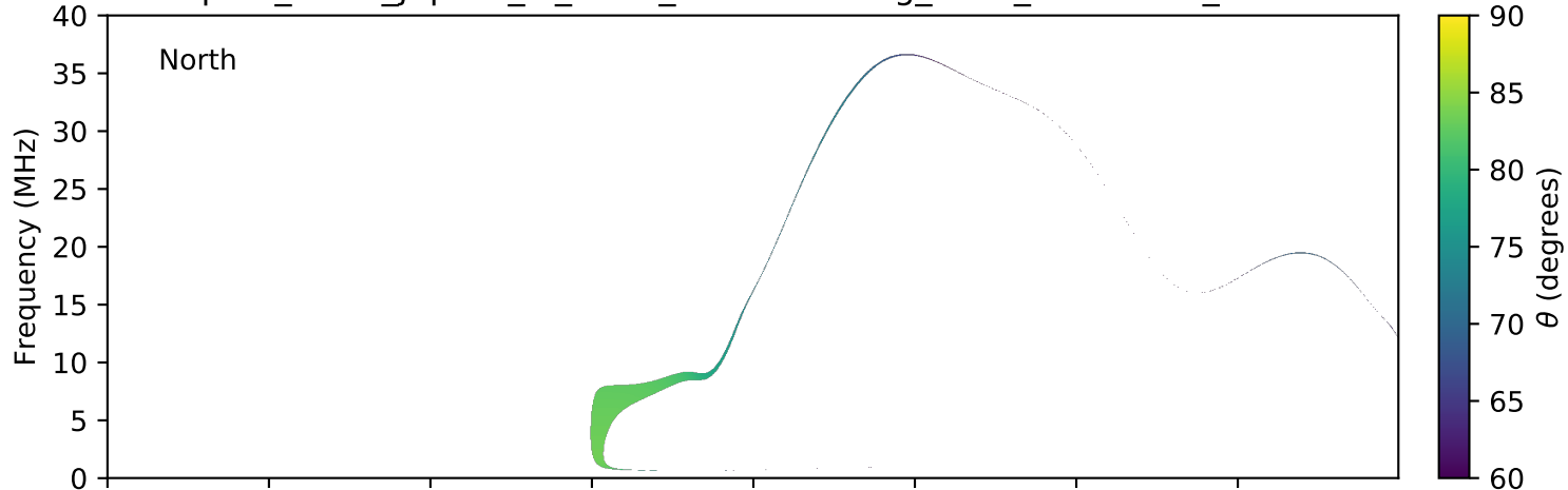
expres_earth_jupiter_io_isaac_lossc-wid1deg_3kev_20100502_v01.cdf
