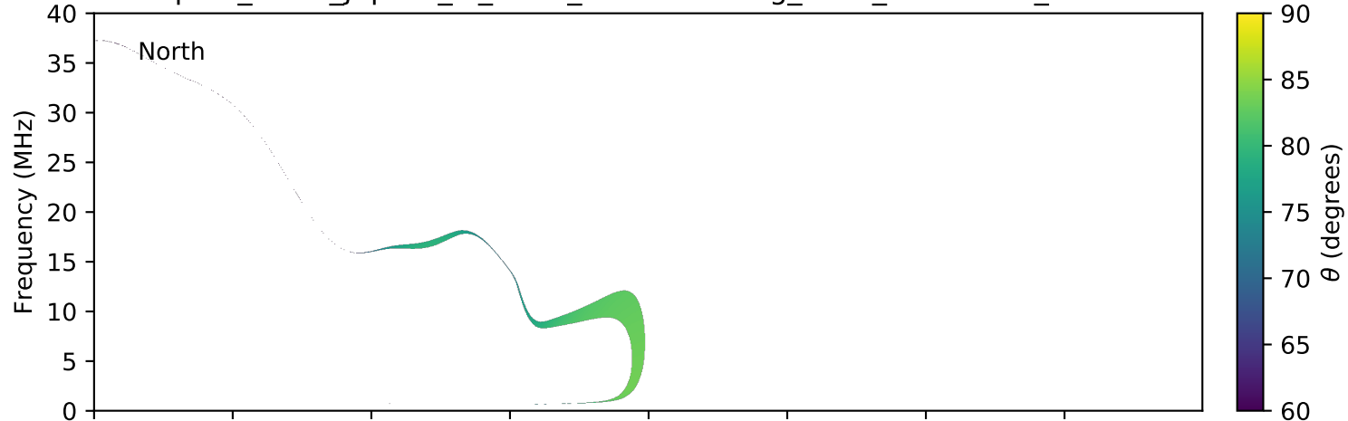
expres_earth_jupiter_io_isaac_lossc-wid1deg_3kev_20100501_v01.cdf
