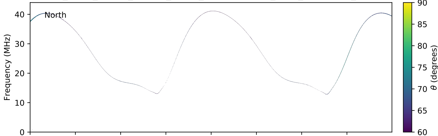
expres_earth_jupiter_europa_jrm09_lossc-wid1deg_3kev_20100531_v01.cdf
