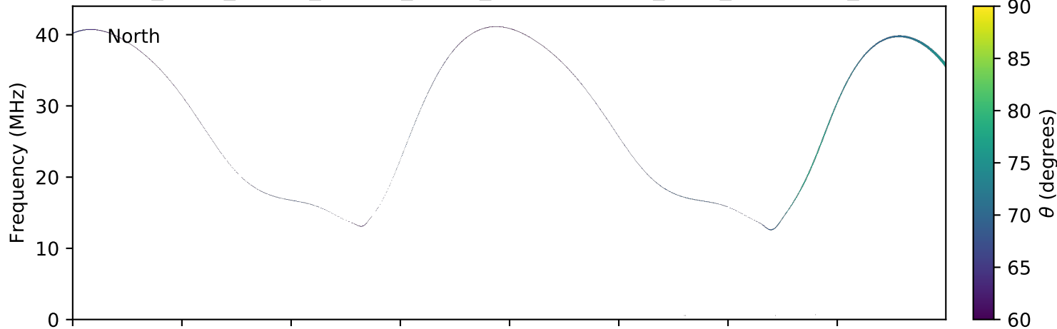
expres_earth_jupiter_europa_jrm09_lossc-wid1deg_3kev_20100524_v01.cdf
