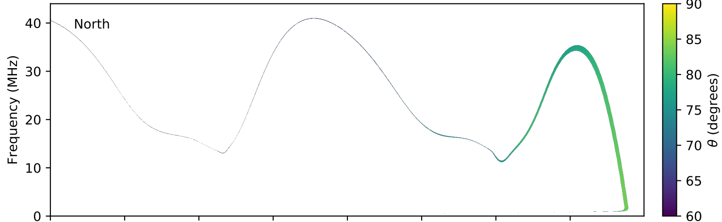
expres_earth_jupiter_europa_jrm09_lossc-wid1deg_3kev_20100510_v01.cdf
