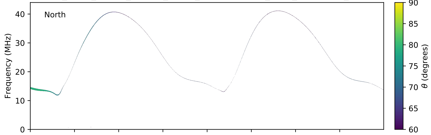
expres_earth_jupiter_europa_jrm09_lossc-wid1deg_3kev_20100506_v01.cdf
