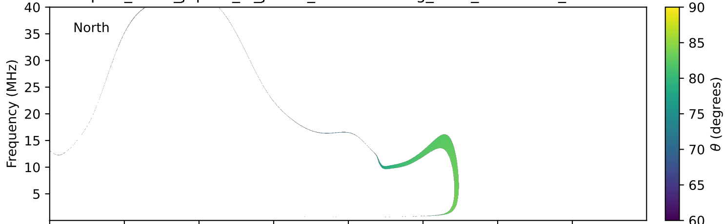
expres_earth_jupiter_io_jrm33_lossc-wid1deg_3kev_20100422_v11.cdf
