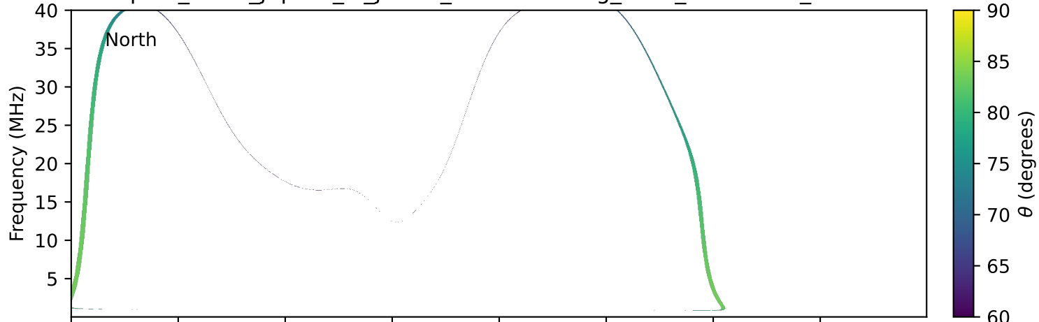
expres_earth_jupiter_io_jrm33_lossc-wid1deg_3kev_20100413_v11.cdf
