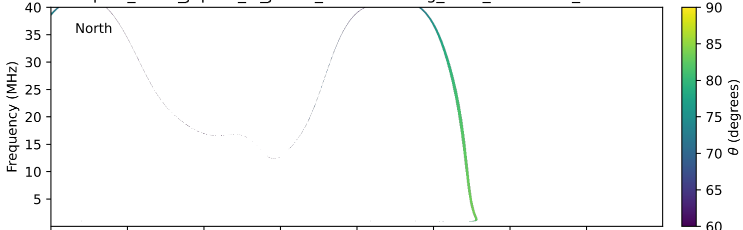
expres_earth_jupiter_io_jrm33_lossc-wid1deg_3kev_20100406_v11.cdf
