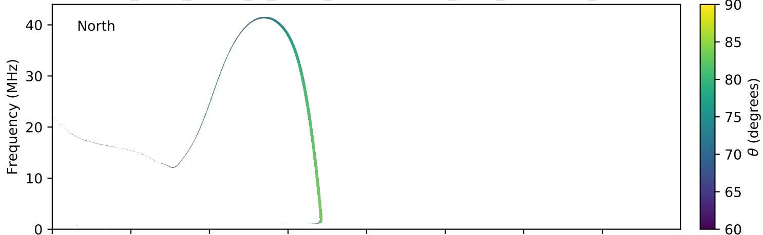
expres_earth_jupiter_io_jrm09_lossc-wid1deg_3kev_20100424_v01.cdf
