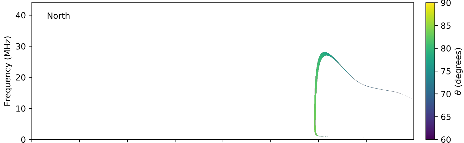
expres_earth_jupiter_io_jrm09_lossc-wid1deg_3kev_20100414_v01.cdf
