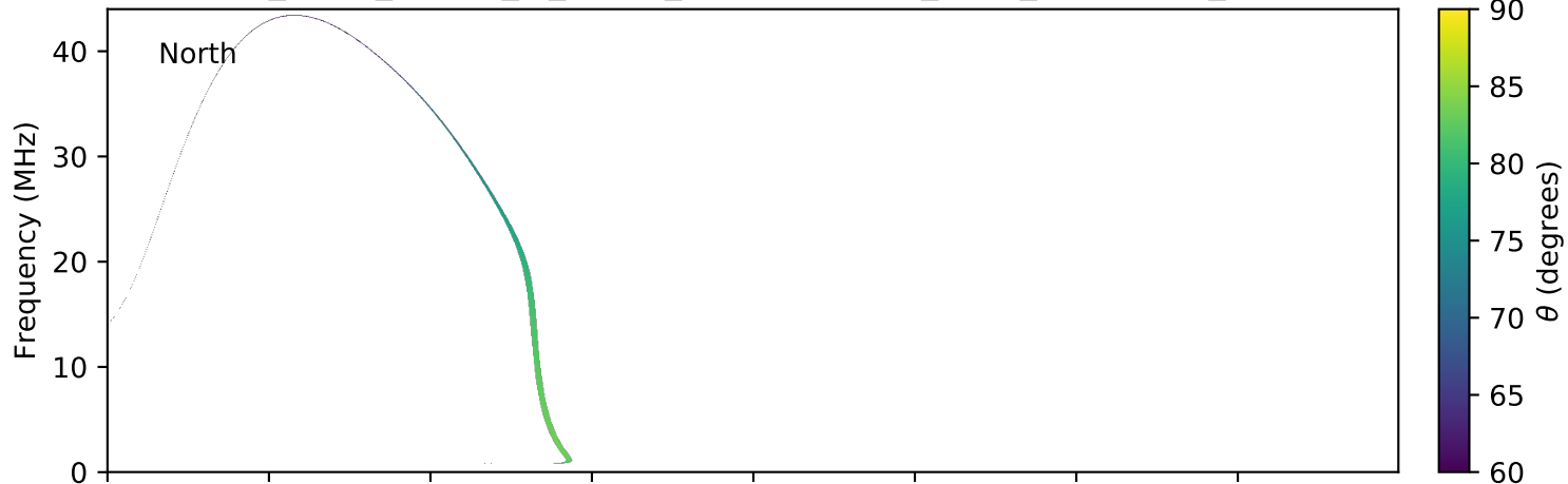
expres_earth_jupiter_io_jrm09_lossc-wid1deg_3kev_20100401_v01.cdf
