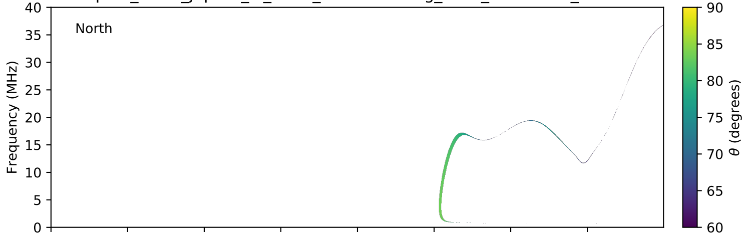
expres_earth_jupiter_io_isaac_lossc-wid1deg_3kev_20100430_v01.cdf
