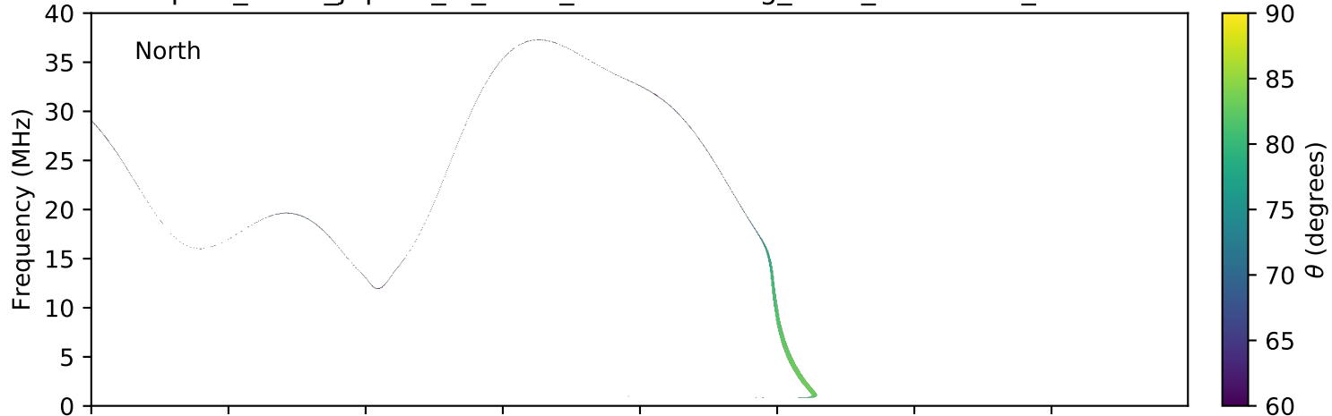
expres_earth_jupiter_io_isaac_lossc-wid1deg_3kev_20100429_v01.cdf
