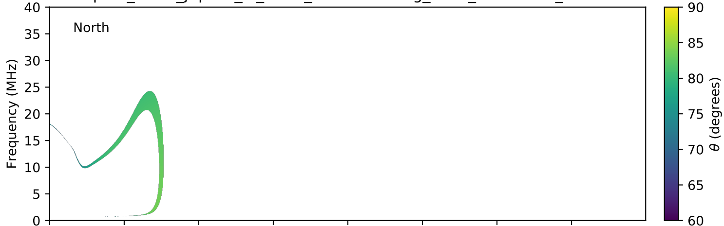
expres_earth_jupiter_io_isaac_lossc-wid1deg_3kev_20100426_v01.cdf
