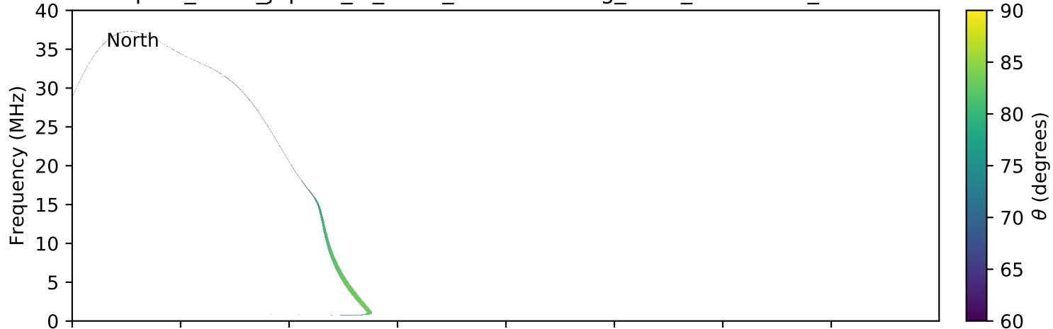
expres_earth_jupiter_io_isaac_lossc-wid1deg_3kev_20100424_v01.cdf
