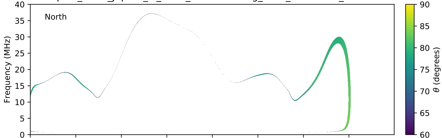
expres_earth_jupiter_io_isaac_lossc-wid1deg_3kev_20100420_v01.cdf
