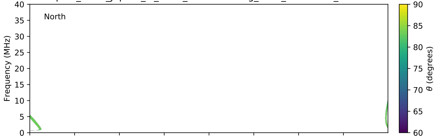
expres_earth_jupiter_io_isaac_lossc-wid1deg_3kev_20100419_v01.cdf
