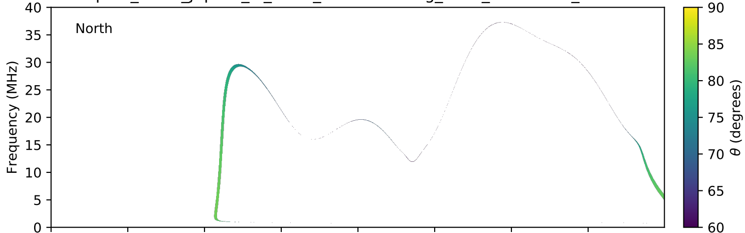
expres_earth_jupiter_io_isaac_lossc-wid1deg_3kev_20100418_v01.cdf
