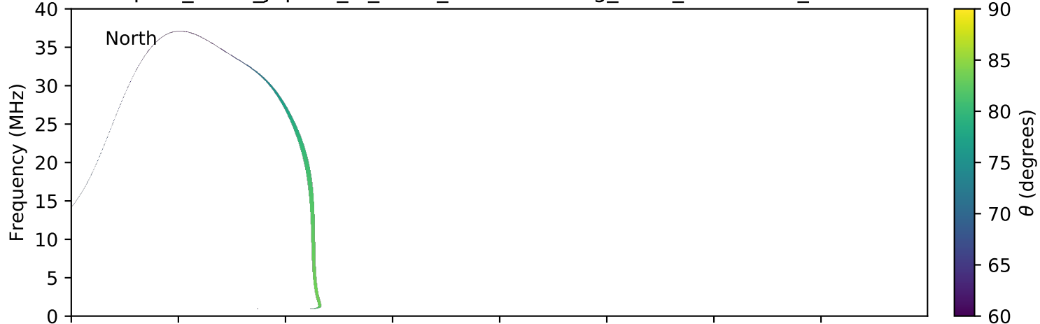
expres_earth_jupiter_io_isaac_lossc-wid1deg_3kev_20100417_v01.cdf
