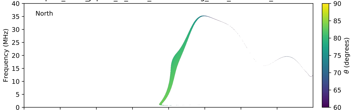
expres_earth_jupiter_io_isaac_lossc-wid1deg_3kev_20100416_v01.cdf
