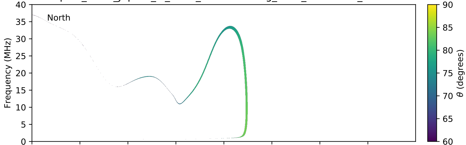
expres_earth_jupiter_io_isaac_lossc-wid1deg_3kev_20100415_v01.cdf
