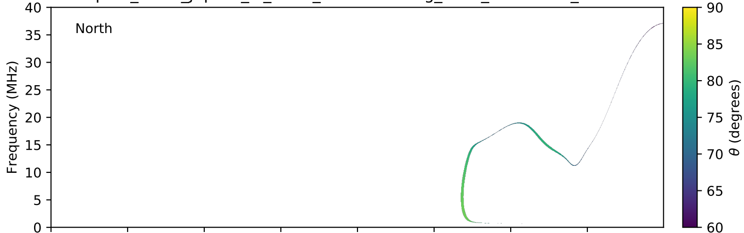
expres_earth_jupiter_io_isaac_lossc-wid1deg_3kev_20100414_v01.cdf
