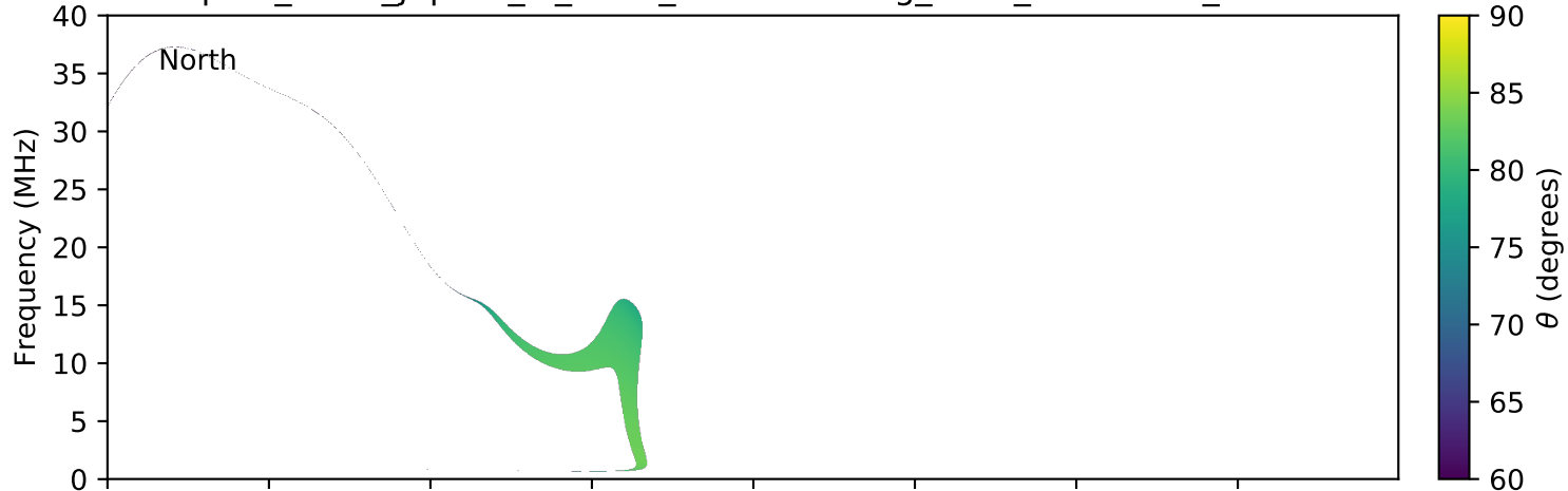
expres_earth_jupiter_io_isaac_lossc-wid1deg_3kev_20100408_v01.cdf
