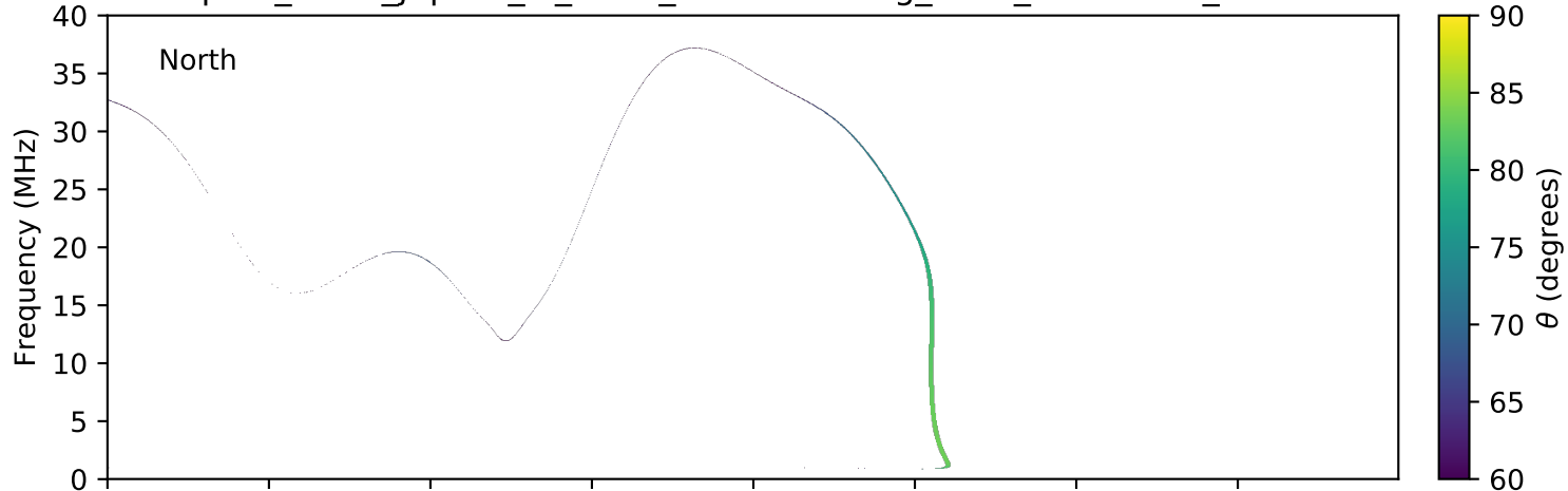
expres_earth_jupiter_io_isaac_lossc-wid1deg_3kev_20100406_v01.cdf
