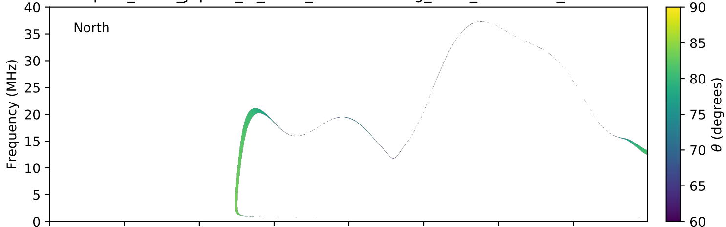
expres_earth_jupiter_io_isaac_lossc-wid1deg_3kev_20100402_v01.cdf
