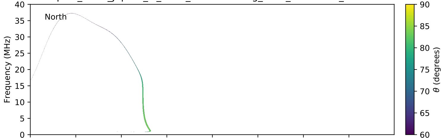
expres_earth_jupiter_io_isaac_lossc-wid1deg_3kev_20100401_v01.cdf
