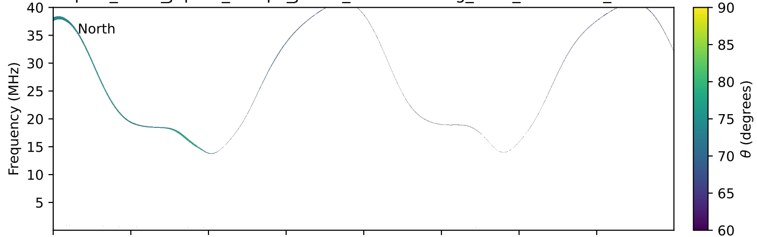
expres_earth_jupiter_europa_jrm33_lossc-wid1deg_3kev_20100411_v11.cdf
