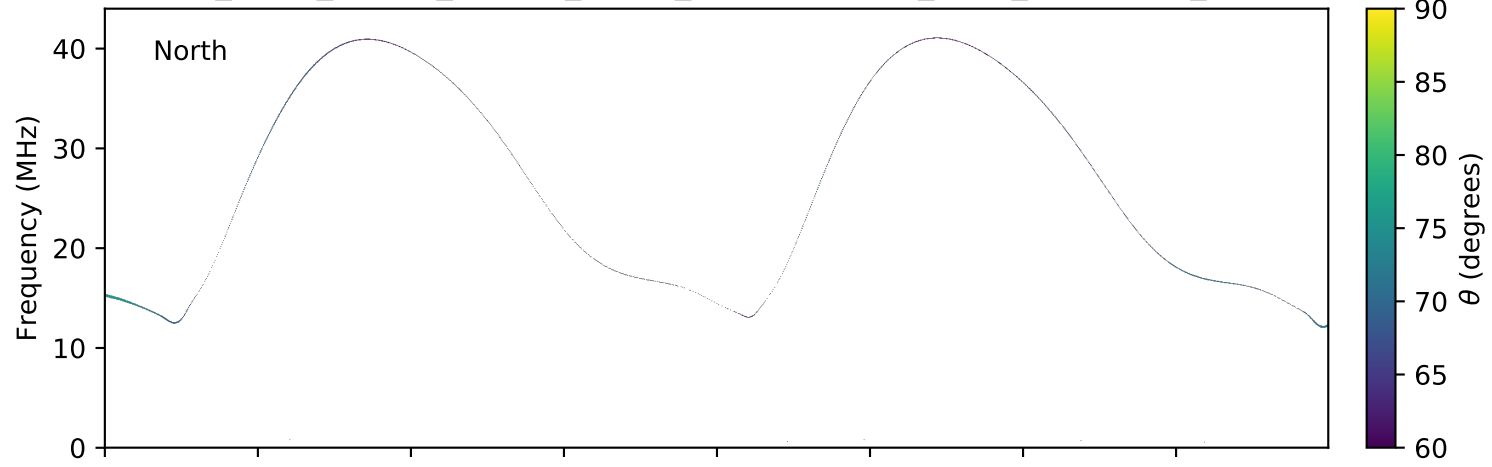
expres_earth_jupiter_europa_jrm09_lossc-wid1deg_3kev_20100429_v01.cdf
