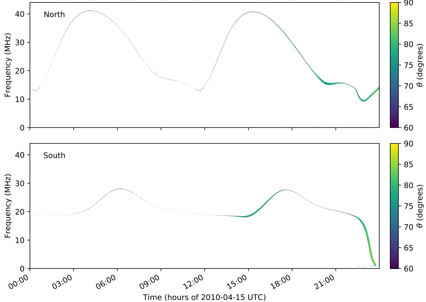
expres_earth_jupiter_europa_jrm09_lossc-wid1deg_3kev_20100415_v01.cdf
