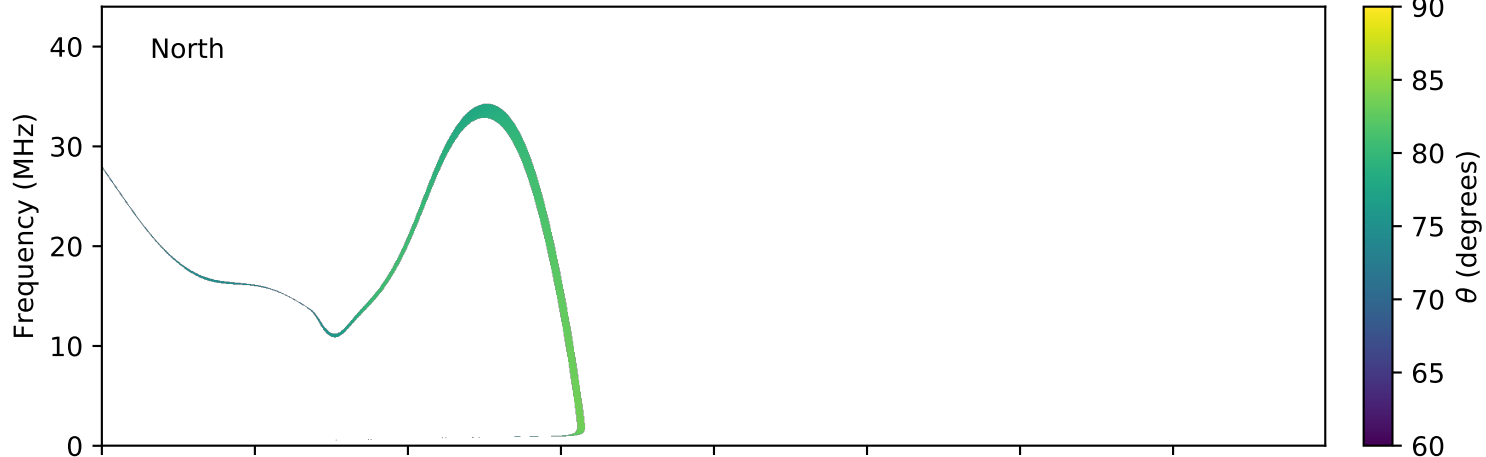
expres_earth_jupiter_europa_jrm09_lossc-wid1deg_3kev_20100405_v01.cdf
