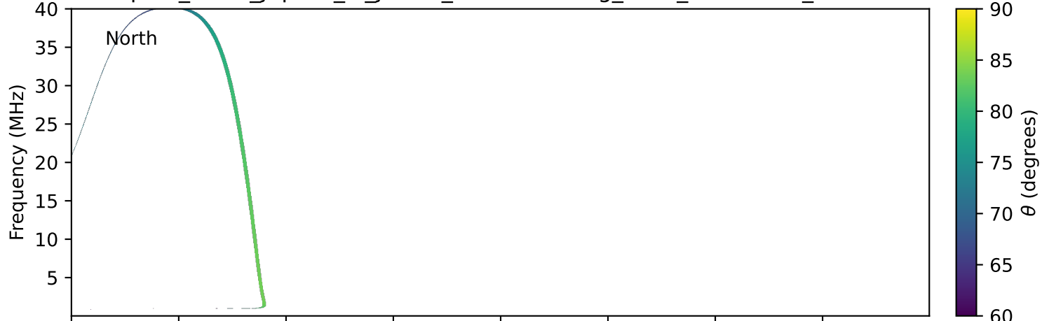
expres_earth_jupiter_io_jrm33_lossc-wid1deg_3kev_20100318_v11.cdf
