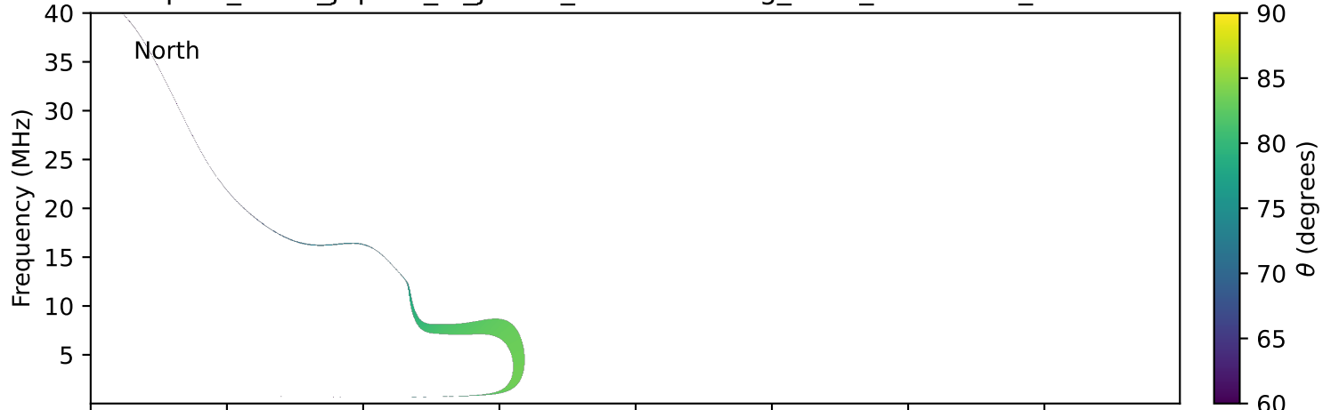
expres_earth_jupiter_io_jrm33_lossc-wid1deg_3kev_20100309_v11.cdf
